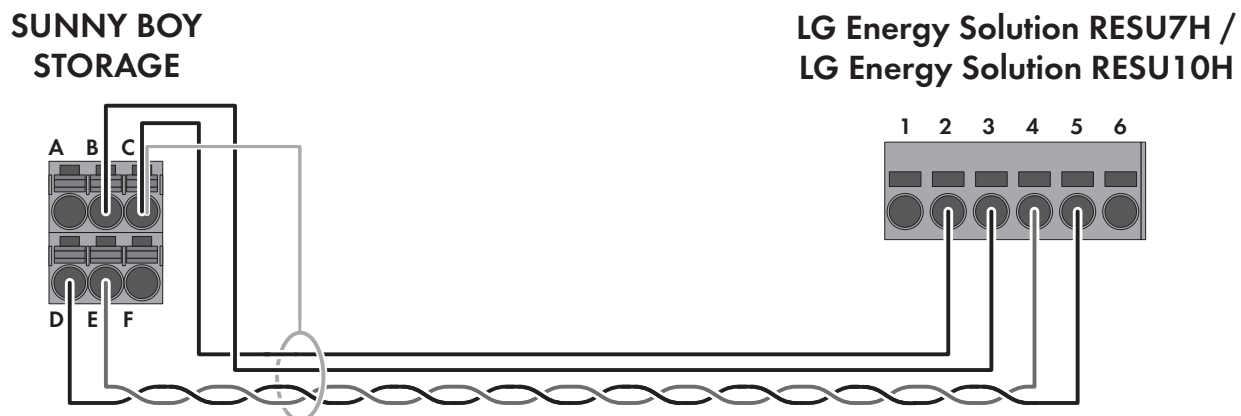
Figure 1: Cabling plan SBS2.5-1VL-10 with RESU7H / RESU10H
