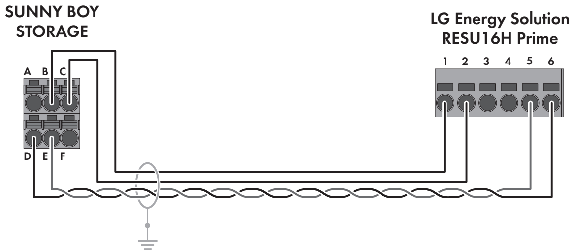
Figure 12: Cabling plan SBS3.8-US-10 / SBS5.0-US-10 / SBS6.0-US-10 with RESU16H Prime
