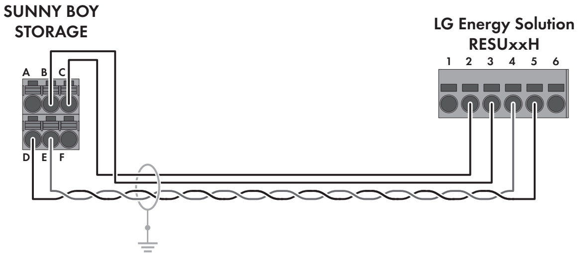
Figure 10: Cabling plan SBS3.8-US-10 / SBS5.0-US-10 / SBS6.0-US-10 with RESU7H / RESU10H
