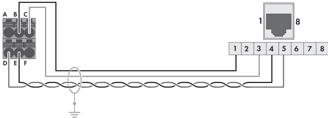
Figure 5: Cabling plan SBS3.7-10 with RESU10M
