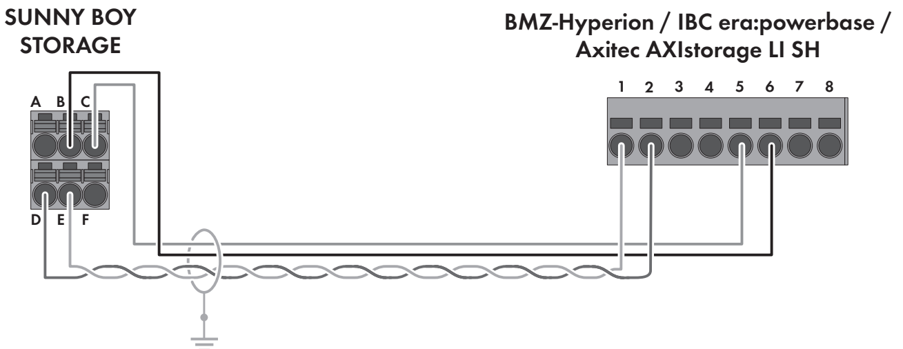
Figure 9: Cabling plan SBS3.7-10 / SBS5.0-10 / SBS6.0-10 with BMZ Hyperion, IBC era:powerbase and Axitec AXIstorage Li SH
